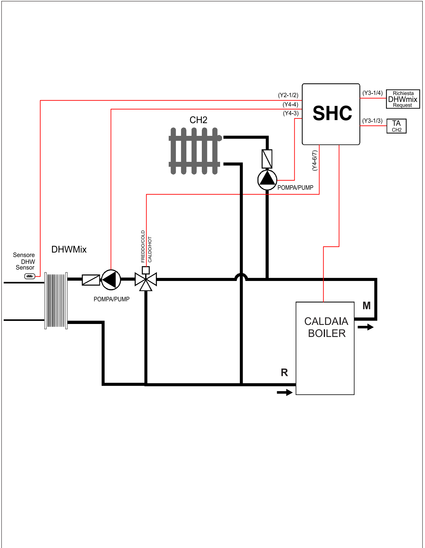
Diagram with 1 plate heat exchanger for mixed domestic hot water and 1 high temperature zone Parameter St ( cod. 309) = 2.
