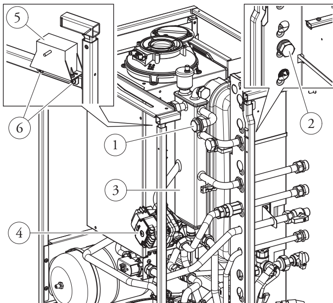
STANDARD BOILER
