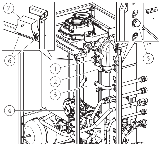
STANDARD BOILER
