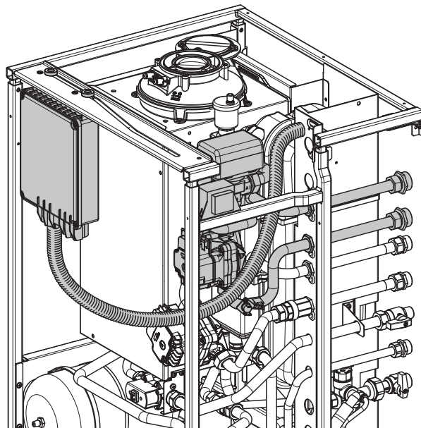
BOILER WITH OPTIONAL KIT
