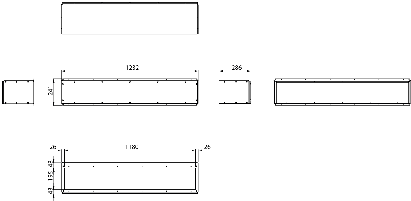
Hydro Vent 5
