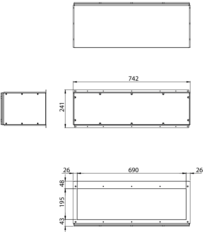
Hydro Vent 3
