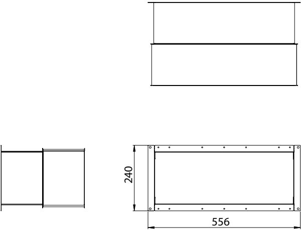
Hydro Vent 2
