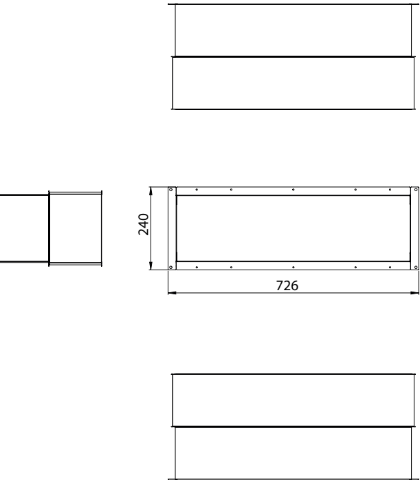
Hydro Vent 3
