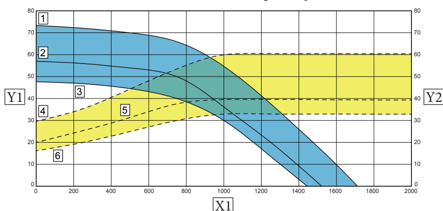
Mixed zone 2 circuit with mixing valve closed
