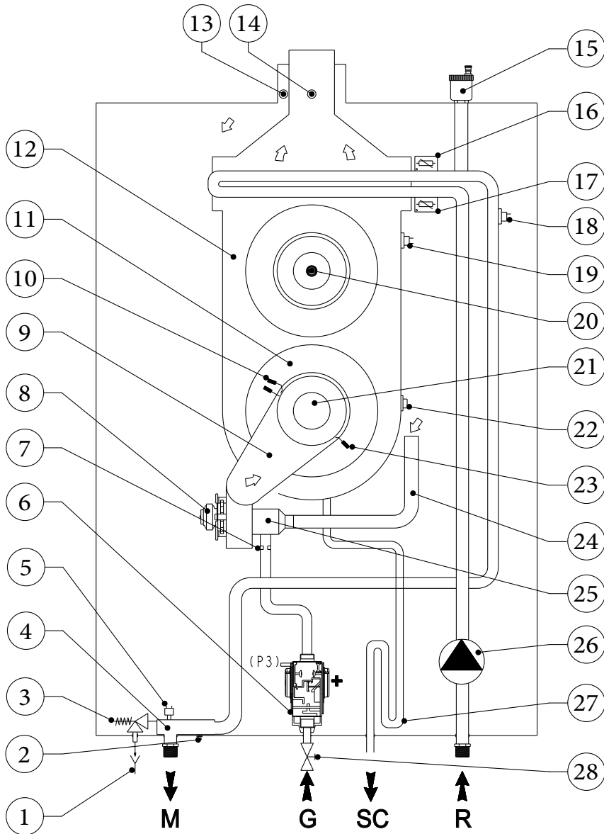
5.1 VICTRIX PRO V2 100 - 120 - 150 EU HYDRAULIC DIAGRAM
